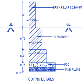
FOOTING DETAILS
