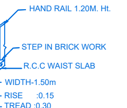
STAIR DETAIL
