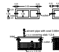
Details of septic tank & trench
