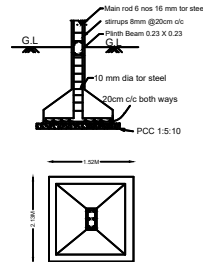
Details of column footing
