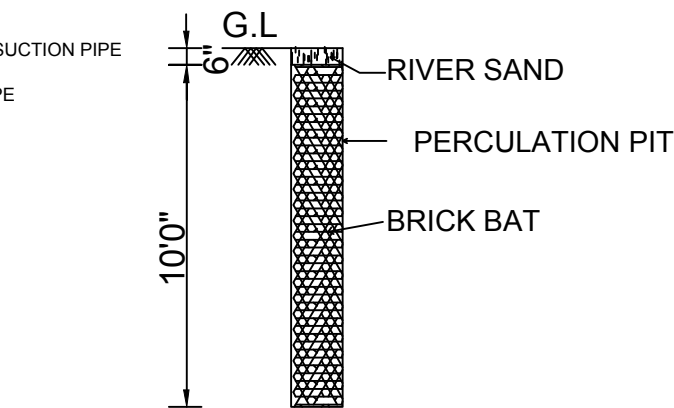
PERCULATION PIT
