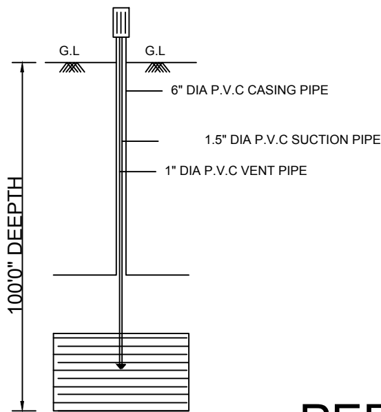
BORE WELL
