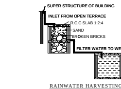
RAINWATER HARVESTING
