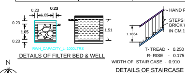
DETAILS OF FILTER BED & WELL
