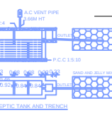
SEPTIC TANK AND TRENCH
