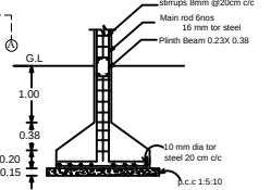
Details of COLUMN
