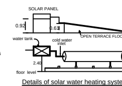
Details of solar water heating system
