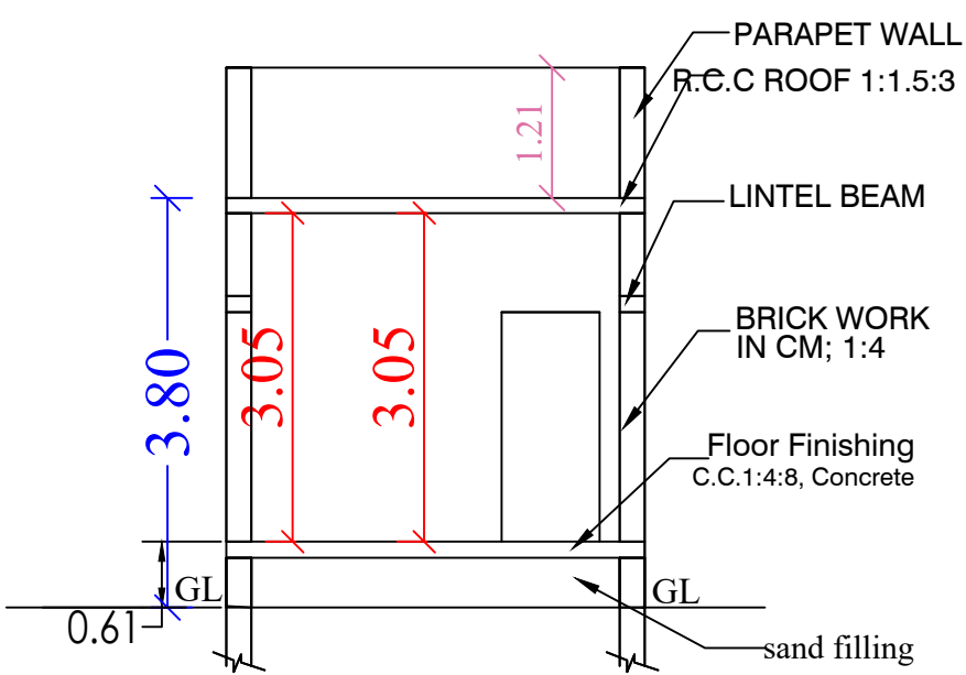
SECTION NN
