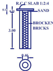
PERCOLATION PIT
