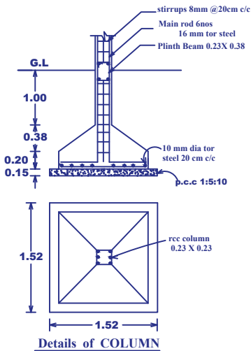
Details of COLUMN
