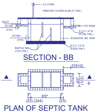
PLAN OF SEPTIC TANK
