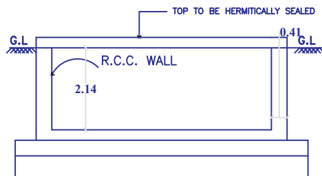
RWHS SECTION (SAMPLE) RWHS_CAPACITY_L=2000LTRS
