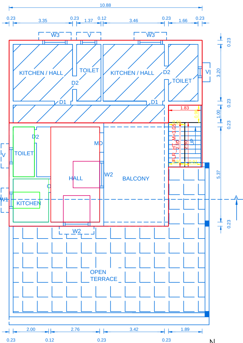
EXG & PROP. FIRST FLOOR PLAN
