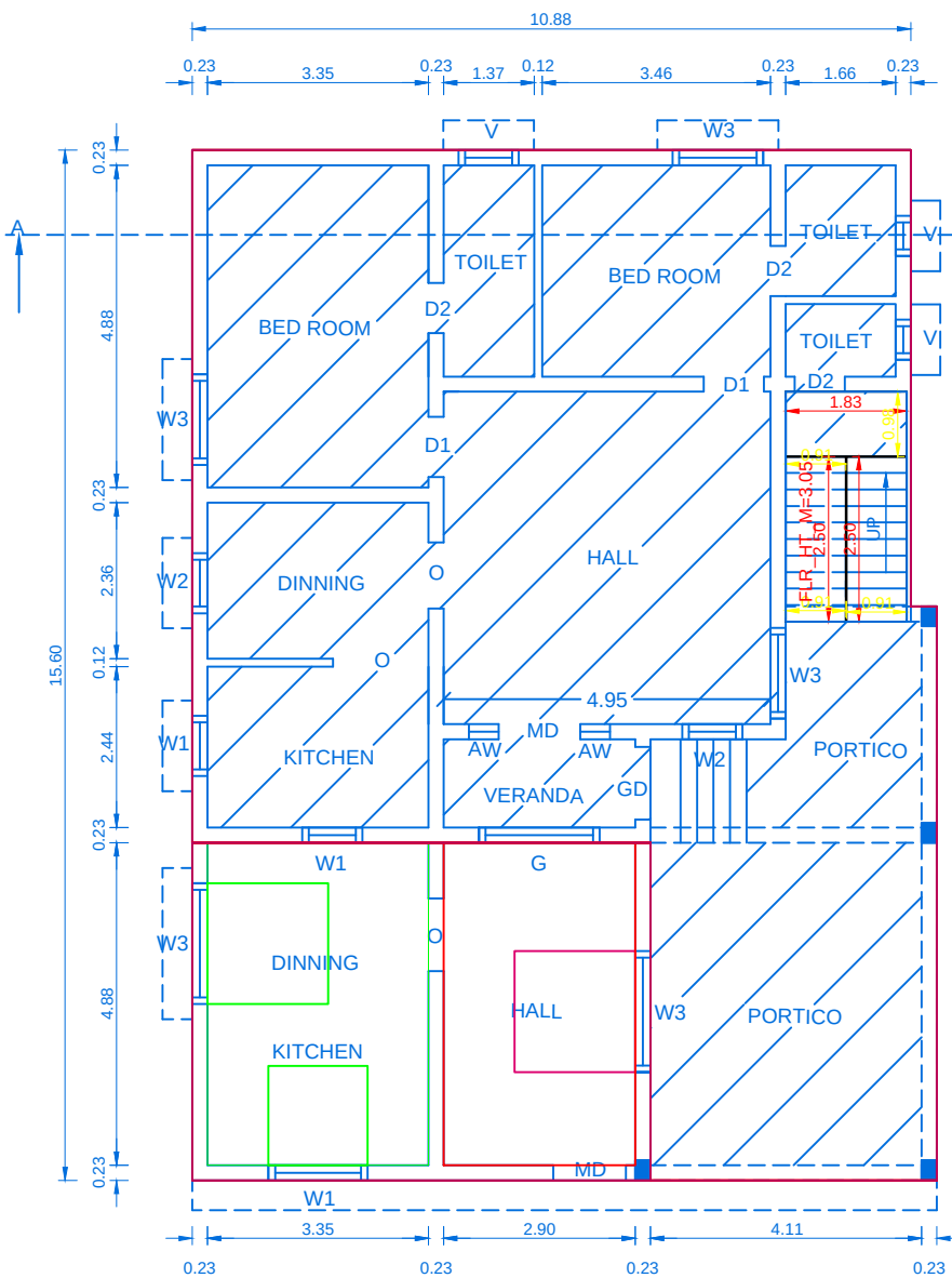
EXG & PROP. GROUND FLOOR PLAN
