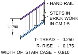
DETAILS OF STAIRCASE
