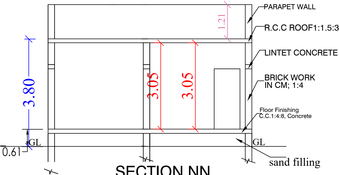
SECTION NN
