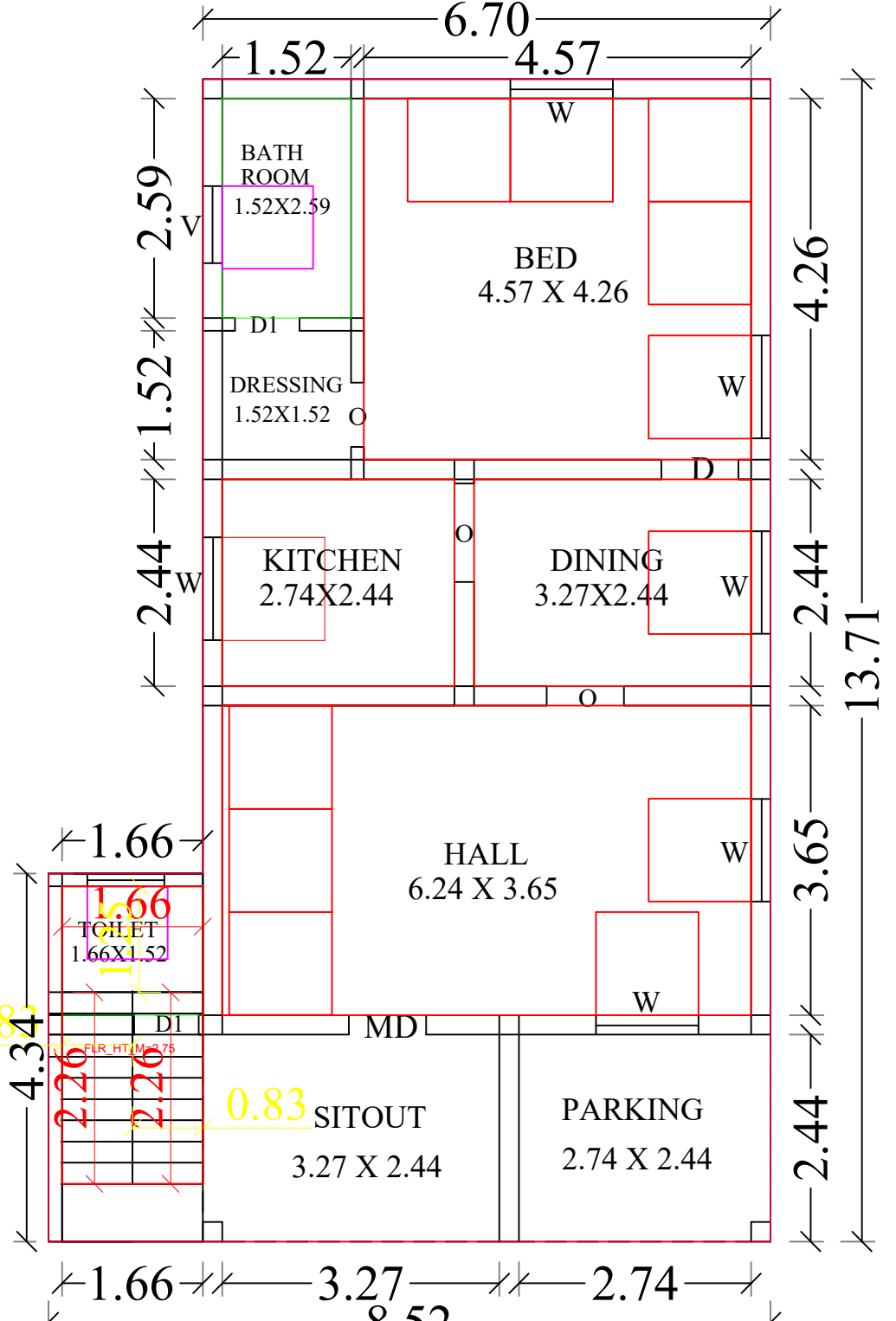
FLOOR PLAN
