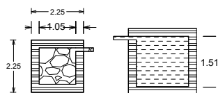
RWH_CAPACITY_L=1000LTRS DETAILS OF FILTER BED & WELL
