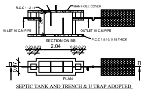
SEPTIC TANK AND TRENCH &amp; U TRAP ADOPTED
