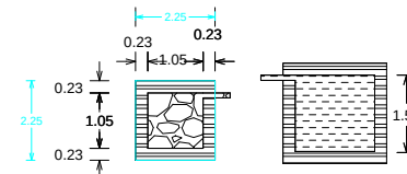
DETAILS OF FILTER BED & WELL
