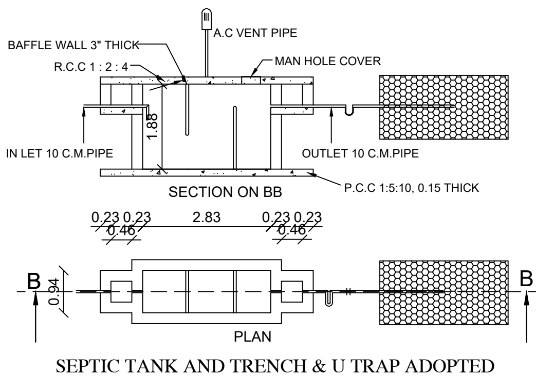
SEPTIC TANK AND TRENCH & U TRAP ADOPTED
