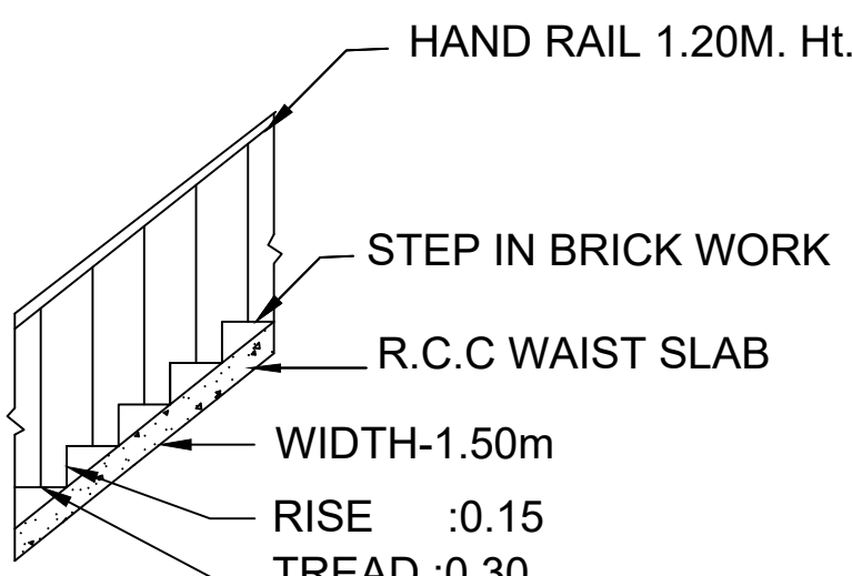
STAIR DETAIL
