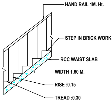
STAIR DETAIL
