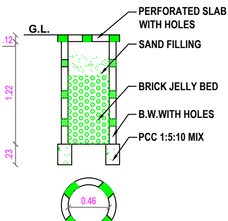
RAIN WATER HARVEST
