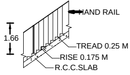
STAIRCASE
