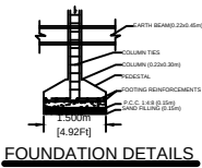
FOUNDATION DETAILS
