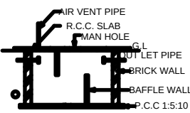
SECTION ON SEP. TANK
