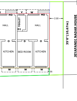
SENTHURAPANDI & PONPANDI HOUSE SITE PLAN (SCALE :- 1:100)
