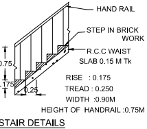
STAIR DETAILS
