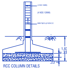
RCC COLUMN DETAILS
