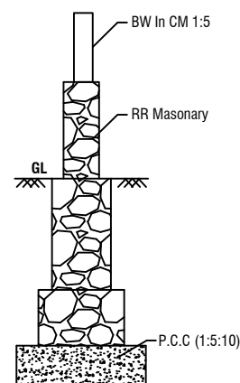
DETAILS OF RR MASONARY
