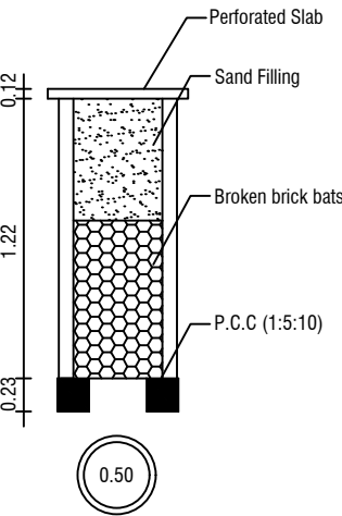
RAIN WATER COLLECTION WELL
