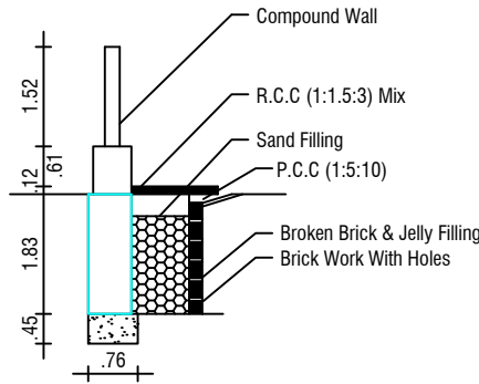
RAIN WATER HARVEST DETAILS
