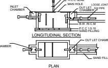
SEPTIC TANK:
