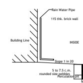
FOUNDATION DETAILS
