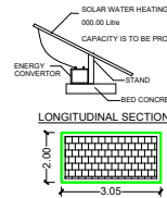
SOLAR SYSTEM
