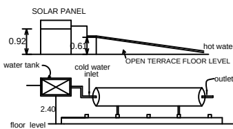
Details of solar water heating system
