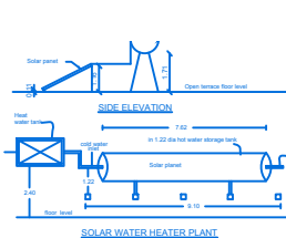
SOLAR WATER HEATER PLANT
