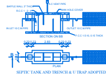
SEPTIC TANK AND TRENCH & U-TRAP ADOPTED
