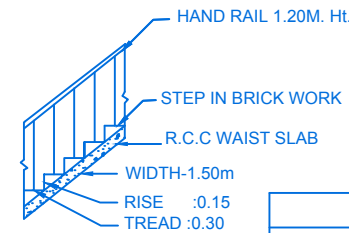
STAIR DETAIL
