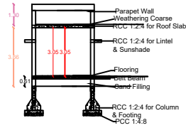
SECTION AB
