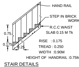
STAIR DETAILS
