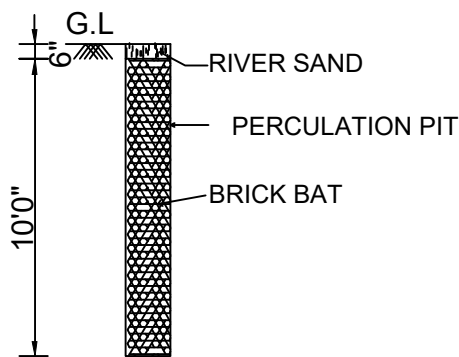
PERCOLATION PIT
