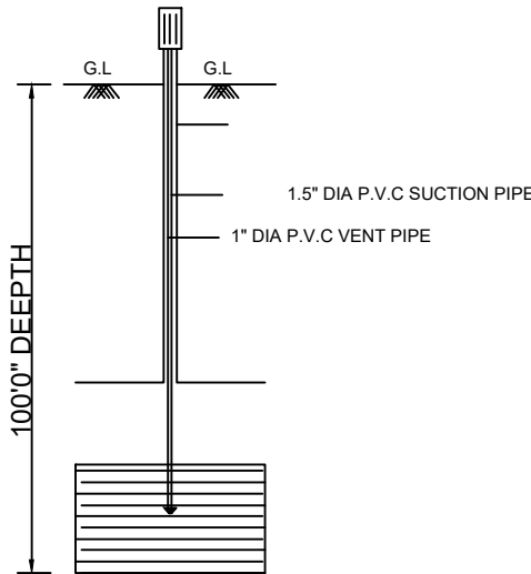
BORE WELL
