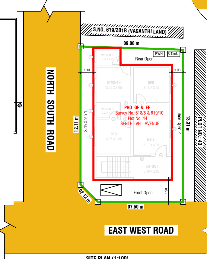
SITE PLAN (1:100)
