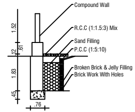
RAIN WATER HARVEST DETAILS
