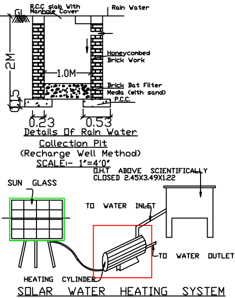
SOLAR WATER HEATING SYSTEM
