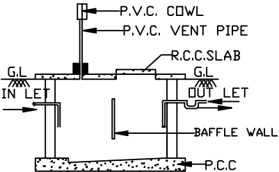
SEC. OF SEPTIC TANK
