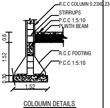
Column Details
