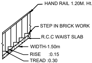
STAIR DETAIL
