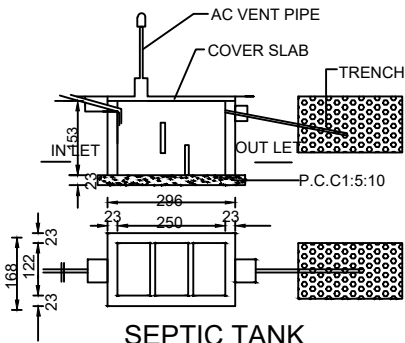
SEPTIC TANK
