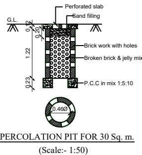
RAINWATER HARVESTING
