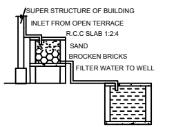
RAINWATER HARVESTING
