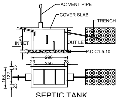
SEPTIC TANK
