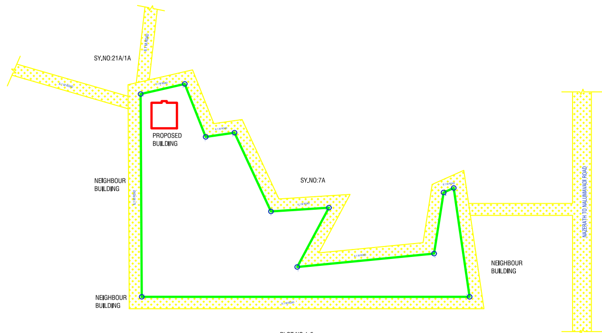
SITE PLAN
