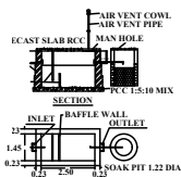
SEPTIC TANK DETAILS
