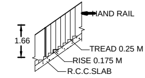
STAIRCASE
