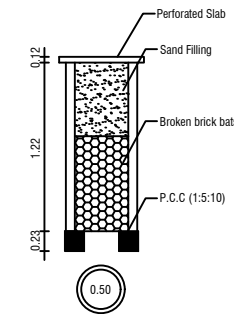
RAIN WATER COLLECTION WELL
