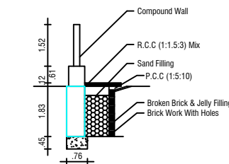
RAIN WATER HARVEST DETAILS
