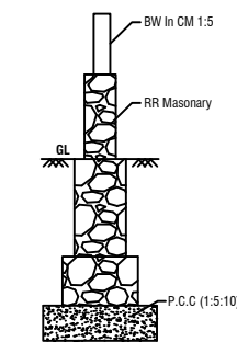
DETAILS OF RR MASONARY
