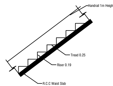
STAIR DETAILS
