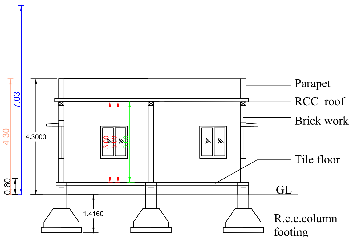
Section -AA
