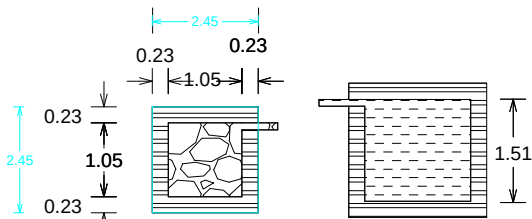
DETAILS OF FILTER BED & WELL
