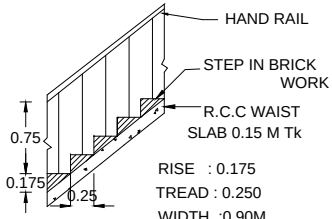
STAIR DETAILS
