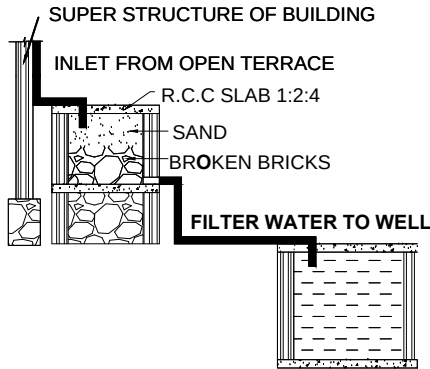
RAINWATER HARVESTING
