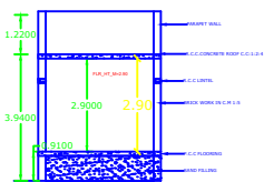
SECTION ON WALL
