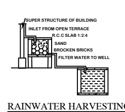
RAINWATER HARVESTING
