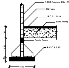
COLUMN DETAIL
