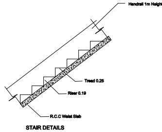
STAIR DETAILS
