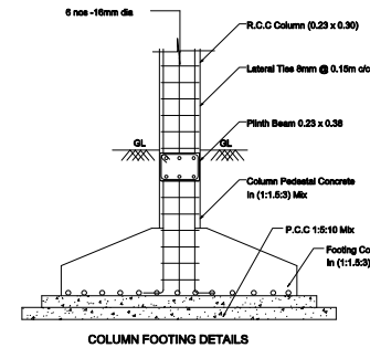
COLUMN FOOTING DETAILS
