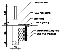
RAIN WATER HARVEST DETAILS
