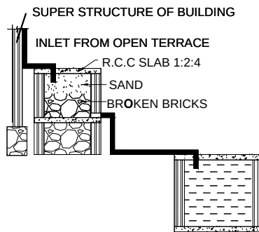
RAINWATER HARVESTING
