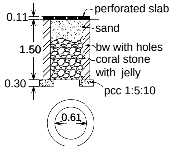
percolation pit
