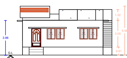
FRONT ELEVATION OF THE PROPOSED BUILDING
