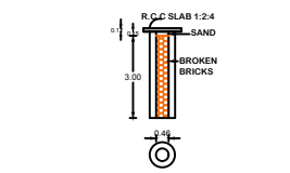
PERCOLATION PIT
