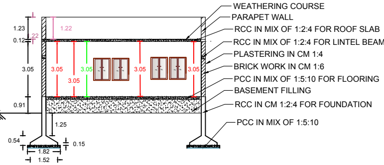
CROSS SECTION A-A' OF THE PROPOSED BUILDING
