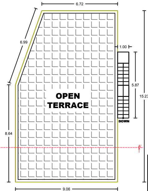
TERRACE PLAN OF THE PROPOSED BUILDING
