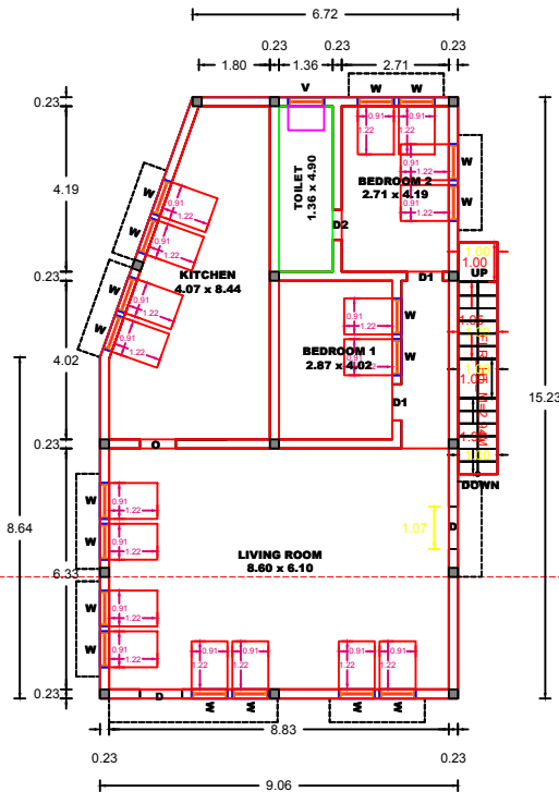
GROUND FLOOR PLAN OF THE PROPOSED BUILDING
