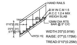
STAIRCASE DETAILS
