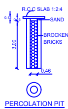
PERCOLATION PIT
