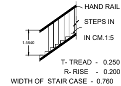
DETAILS OF STAIRCASE
