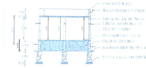
SECTION ON "V-B"
