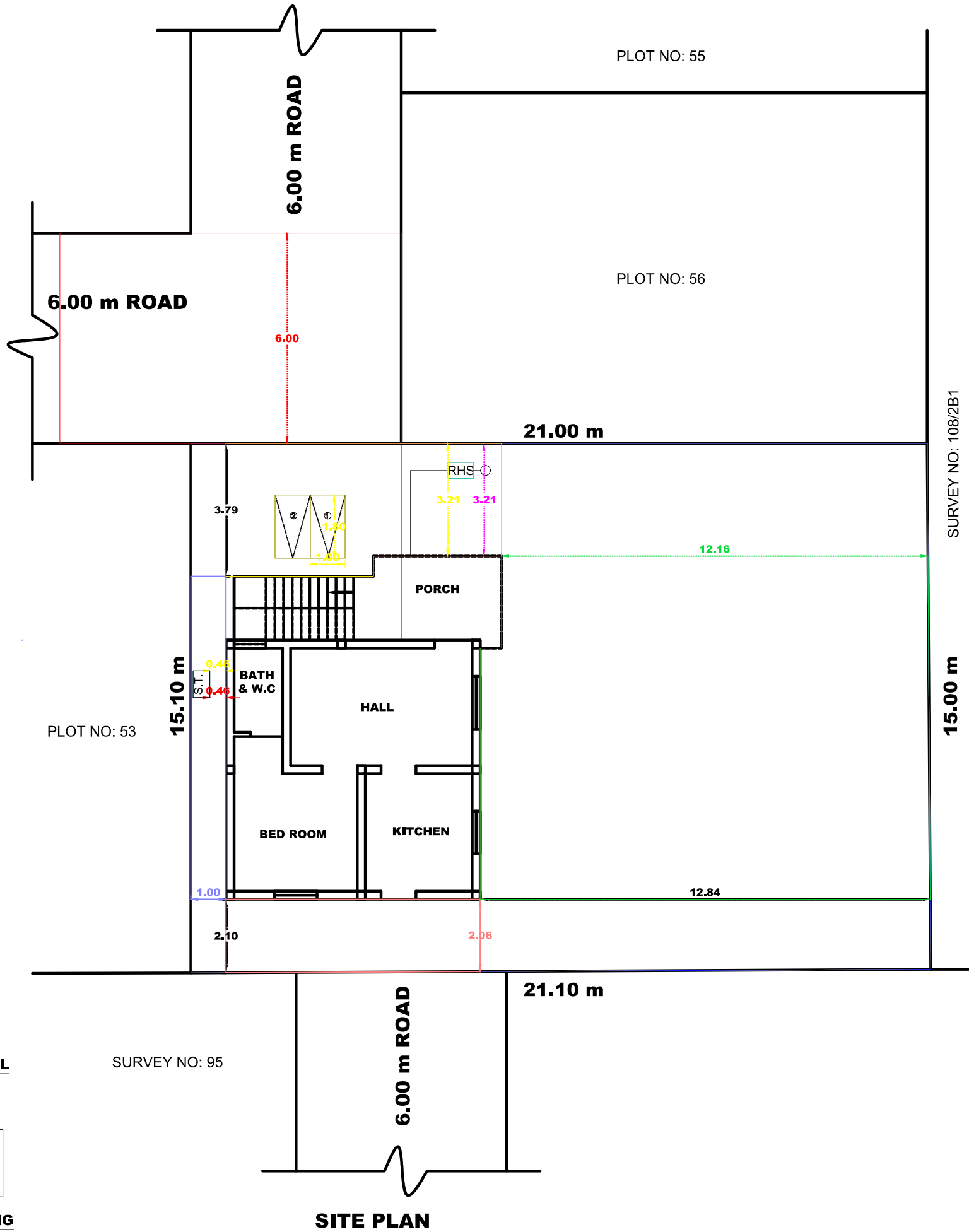
SITE PLAN
