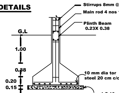
Details of column footing
