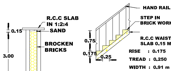
STAIR DETAILS
