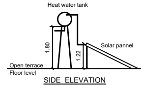
SIDE ELEVATION
