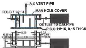
SEPTIC TANK DETAILS
