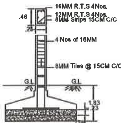
RCC COLUMN DETAILS
