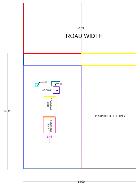
RESIDUARY PLOT SKETCH, SUPER IMPOSED SKETCH (SITE PLAN)
