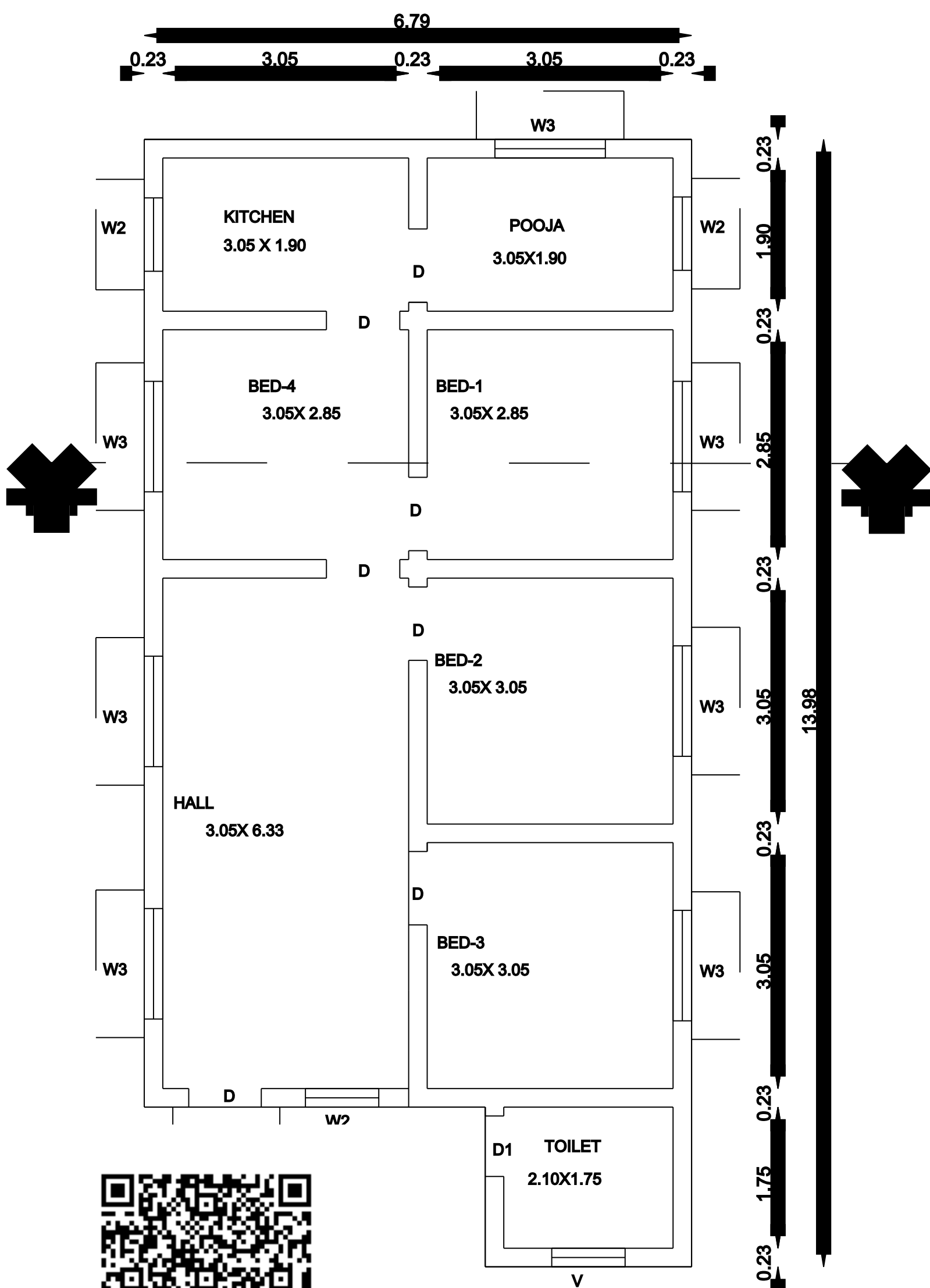
FLOOR PLAN
