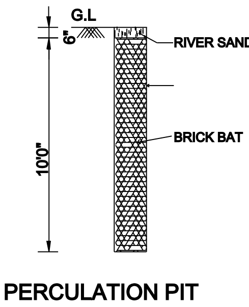
PERCOLATION PIT
