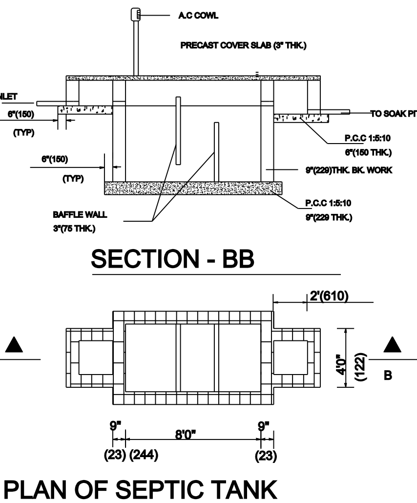
PLAN OF SEPTIC TANK
