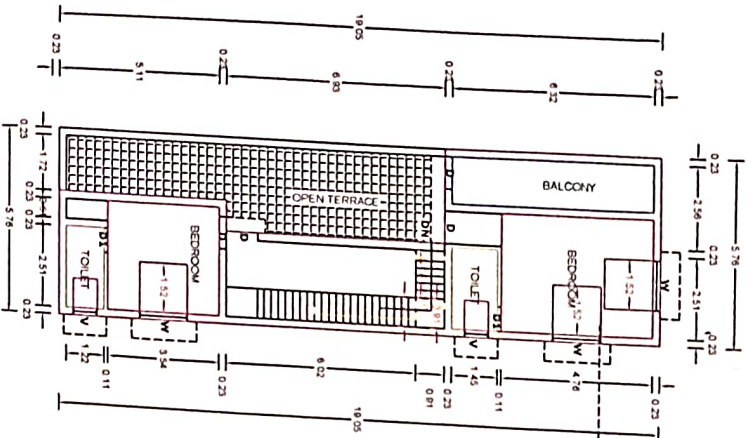
PRO. FIRST FLOOR PLAN
